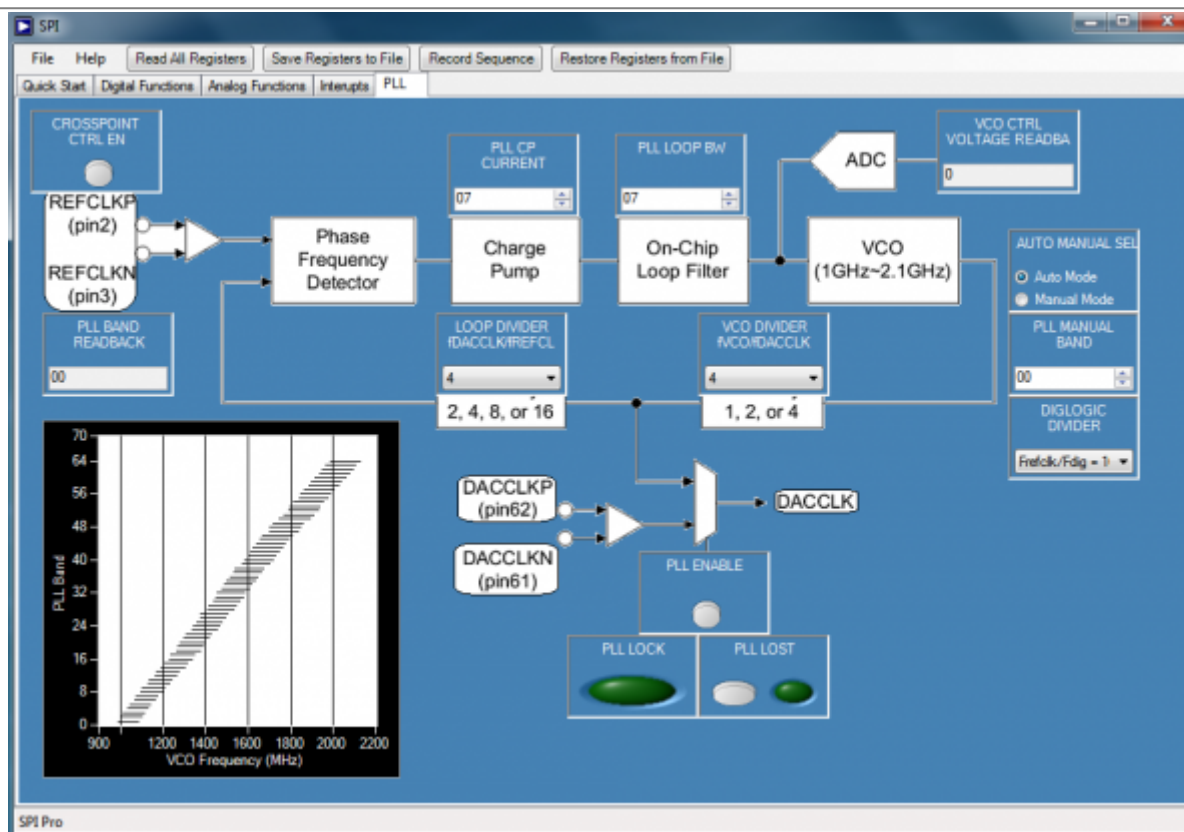
Figure 9 AD9142A SPI PLL Tab
