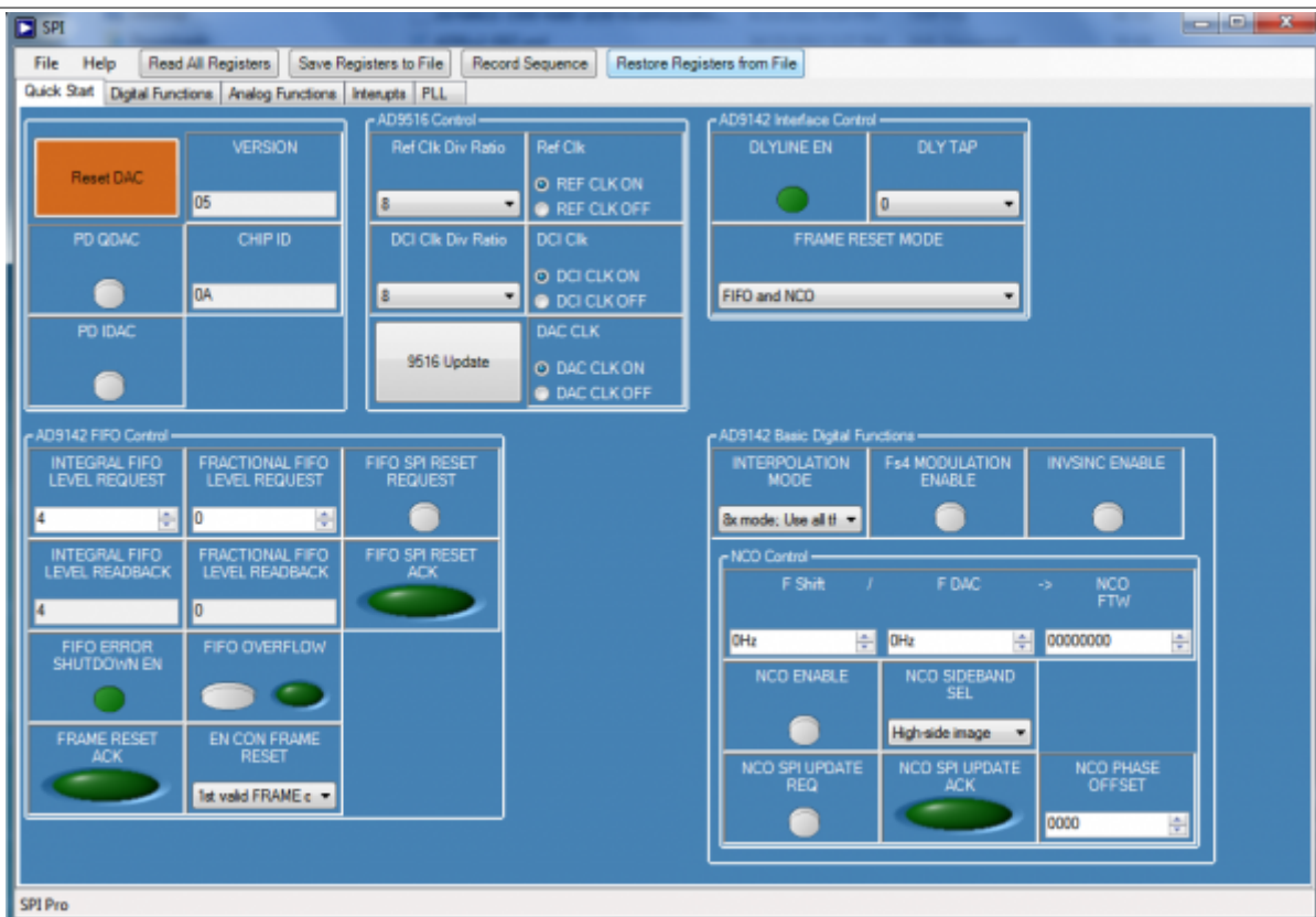
Figure 8 AD9142A SPI Quick Start tab
